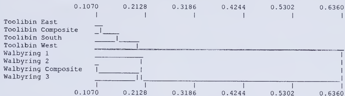
Figure 7. Classification of replicates and composite samples from Toolibin and Walbyring Lakes, showing the similarity of replicates from the same wetland.
